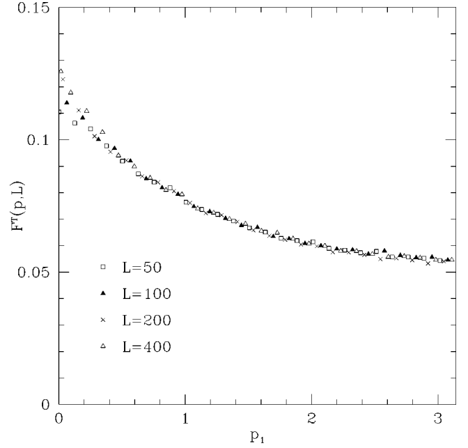
FIG. 2. Transverse current correlation: approach to the thermodynamic limit.
