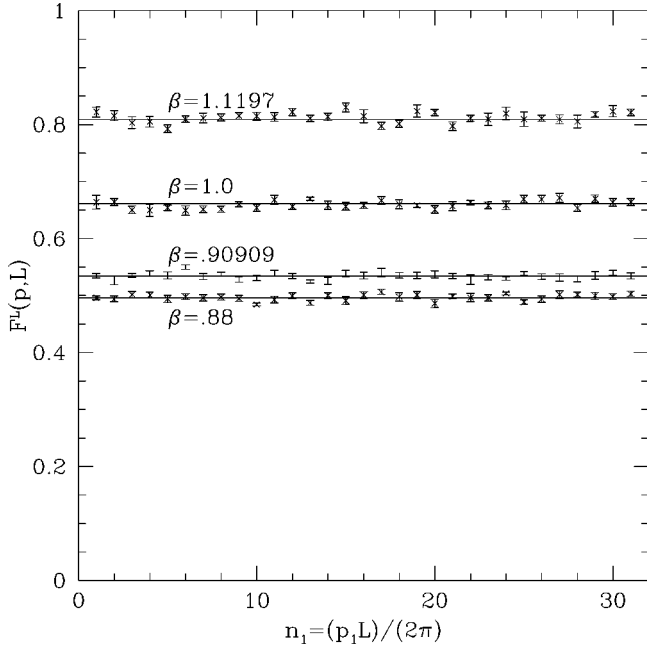
FIG. 1. Longitudinal current correlation.
