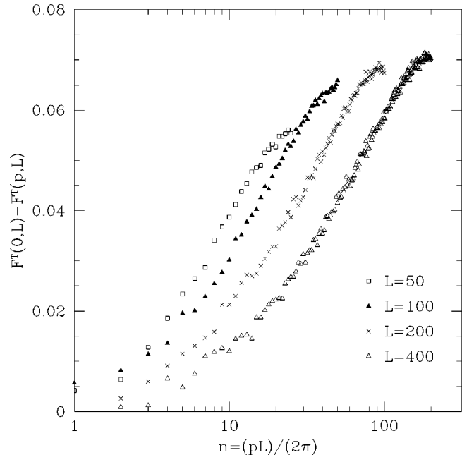
FIG. 3. Transverse current correlation on different lattices.
