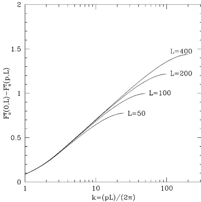
FIG. 4. Transverse free current correlation: approach to the continuum limit.
