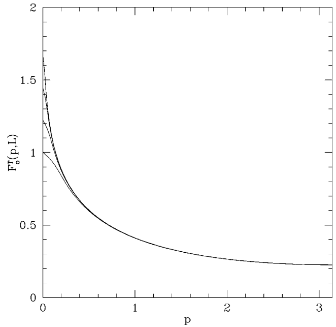
FIG. 5. Transverse free current correlation: approach to the thermodynamic limit.
